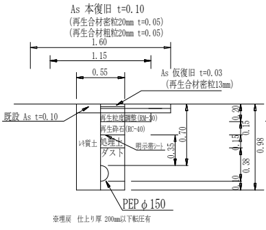
(市道車道部) PEPφ150土工図①
