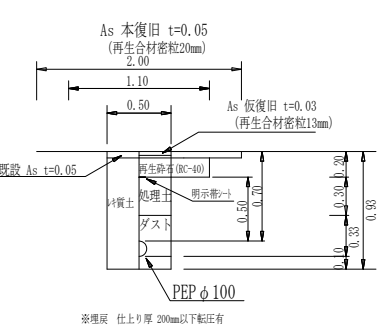
(市道歩道部) PEPφ100土工図④
