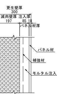
躯体側壁
