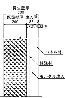
躯体側壁
