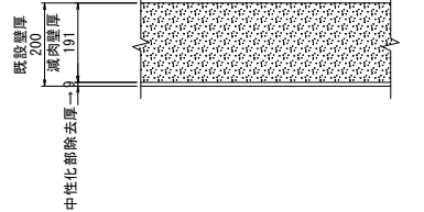
躯体側壁
