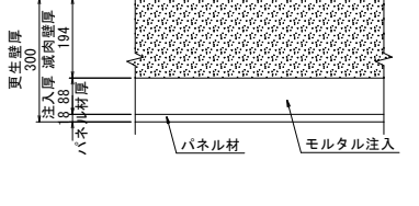
躯体側壁
