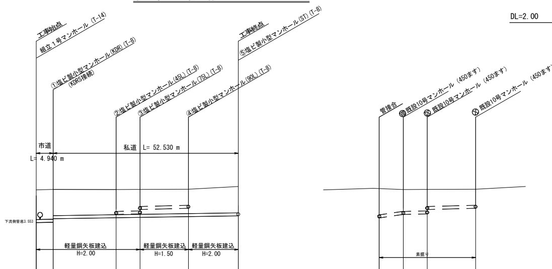
管渠埋設縱断面図 S = \frac{\text{縦}}{\text{横}} = \frac{1}{500}
