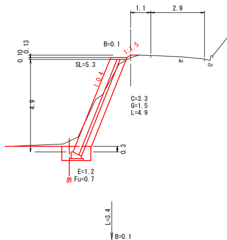
SECT. 0.0 GH=169.61 FH=169.750
